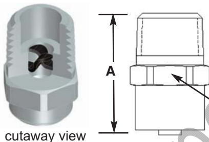
cutaway view
