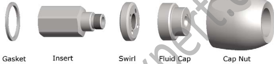
3/4" and 1" SB Nozzle Exploded View
