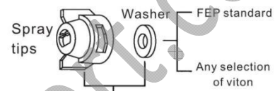
Quick removeable e tips and gasket
