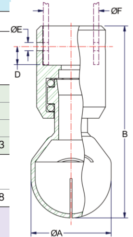
Threaded and Clip On Connections
